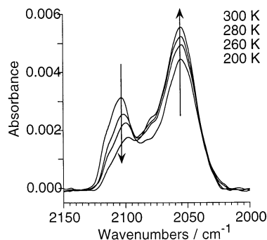
Fig. 8. IR spectrum in the range 2150\text{--}2000 \text{ cm}^{-1} of the \text{Fe}(t\text{-hsbpy})_2(\text{NCS})_2 complex in the LB film on calcium fluoride for various temperatures ( T=200, 260, 280 and 300 \text{ K} ). Arrows indicate the intensity variations for increasing temperature.
