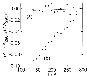
Fig. 3. Temperature dependence of the relative absorbance (A_T - A_{RT})/A_{RT} at 344 nm for the C^c -containing film before (a) and after (b) irradiation at \lambda_{\text{exc}} = 260 nm at 140 K.
