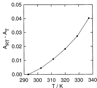
Fig. 7. Temperature dependence of the absorbance A_{RT} - A_T at \lambda_{\text{isobestic}} = 313 nm in the photostationary state (2).
