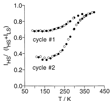
Fig. 9. Ratio I_{\text{HS}}/(I_{\text{HS}} + I_{\text{LS}}) of the integrals of the IR peaks between 2090 and 2135 \text{cm}^{-1} ( I_{\text{LS}} ) and between 2000–2090 \text{cm}^{-1} ( I_{\text{HS}} ) in the LB film versus temperature (see Fig. 8). Open circle: decreasing temperature, full circle: increasing temperature. First thermal cycle: 300 \rightarrow 100 \rightarrow 400 K. Second thermal cycle: 400 \rightarrow 100 \rightarrow 400 K.
