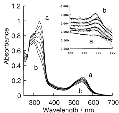
Fig. 6. Evolution of the UV-vis spectrum of 1.9 \times 10^{-5} M acetonitrile solution of \text{C}_{t,v} upon irradiation at 334 nm. (a) Initial spectrum; (b) spectrum of the photostationary state. Inset: corresponding evolution of the absorbance in the d-d transition area; for clarity, all bands were slightly shifted upwards (except a).
